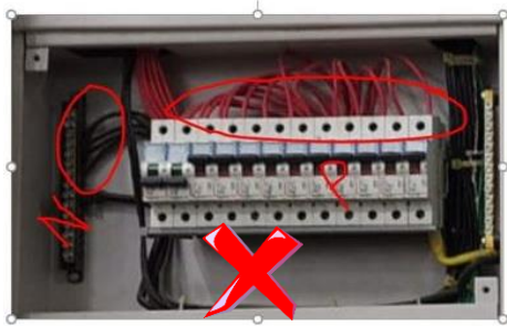
Fig 1. Dedicated neutral for each single-phase circuit
