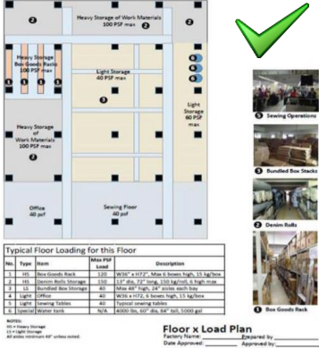
Sample load plan
